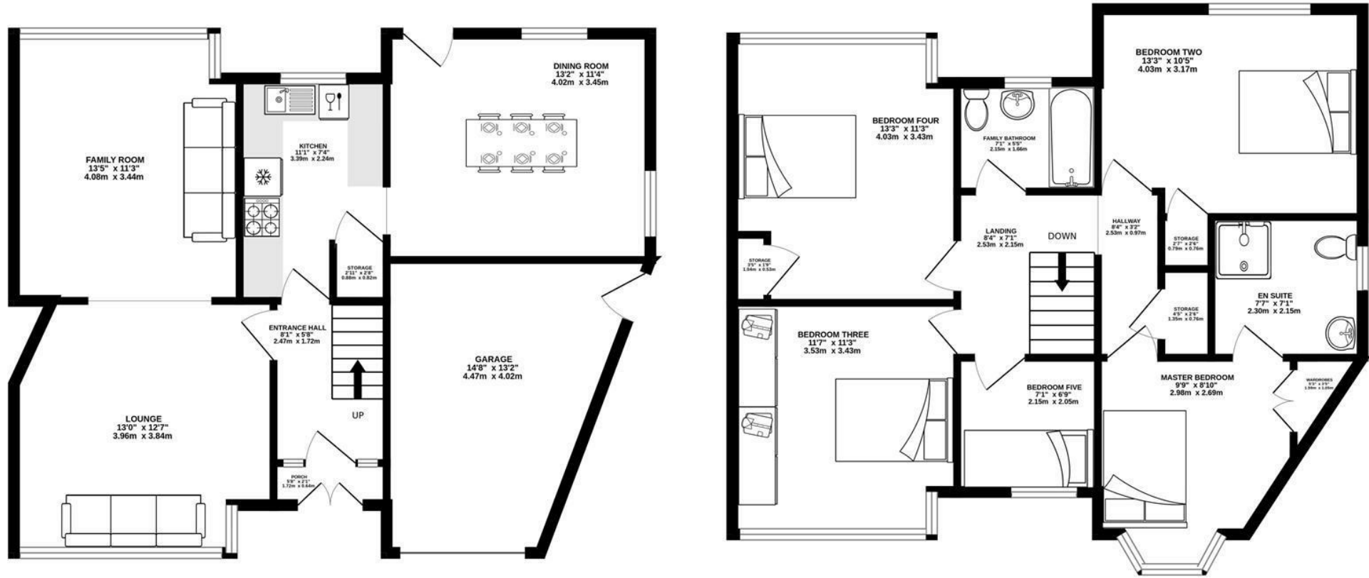
GROUND FLOOR 745 sq.ft. (69.3 sq.m.) approx.
